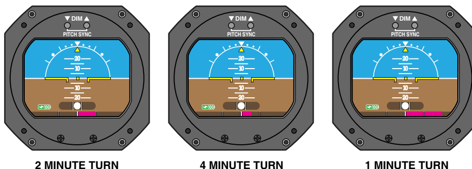
Figure 1.4, Rate of Turn Indication.
