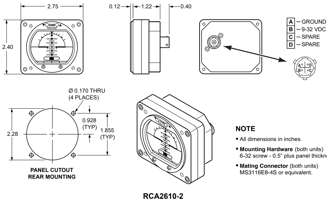
Figure 1.1, General Dimensions
